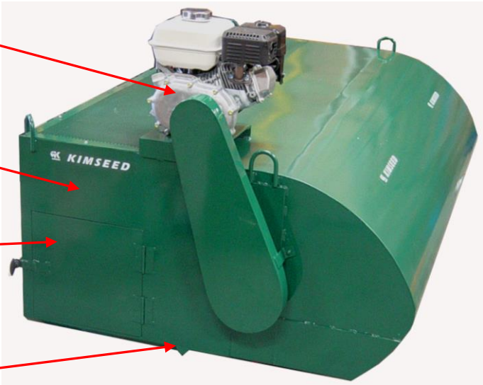
Motor Petrol, Diesel or Hydraulic
