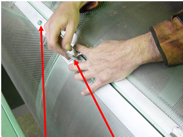
Replacing Screens by Undoing Clips and then nuts and Bolts
