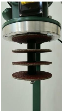
The 4 Scarifying Discs in situ.
